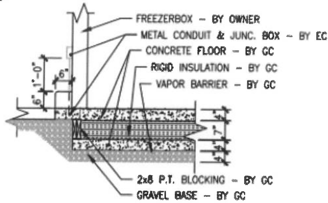
CROSS SECTION AT THRESHOLD
