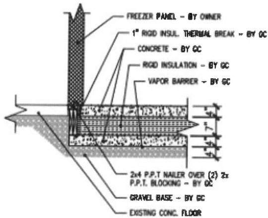
1 FREEZER SLAB DETAIL SCALE: 3/8" = 1'-0"
