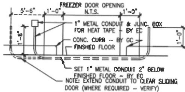
ELEVATION AT DOOR OPENING
